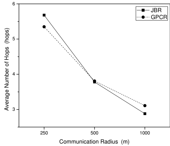
Figure 9: Average number of hops over the Communication Radius.
