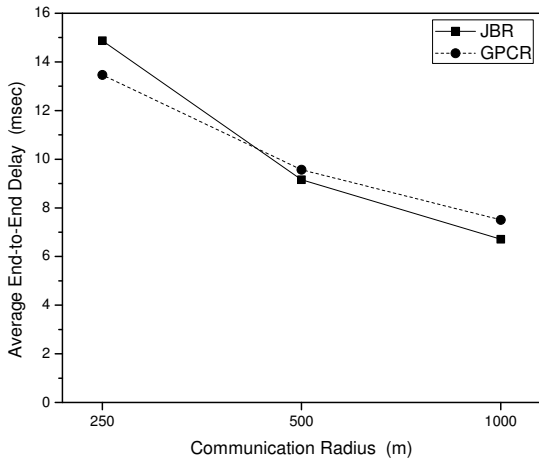
Figure 6: Average End-to-end delay over the Communication Radius.
