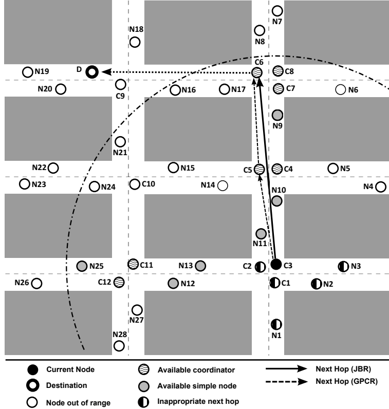
Figure 1: Greedy forwarding from a coordinator.
