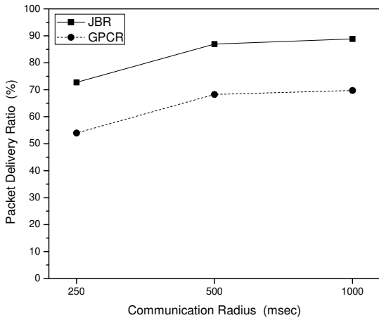
Figure 8: Packet Delivery Ratio over the Communication Radius.
