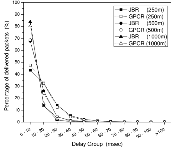
Figure 7: Packet Delay Distribution, as a percentage of the total delivered packets.
